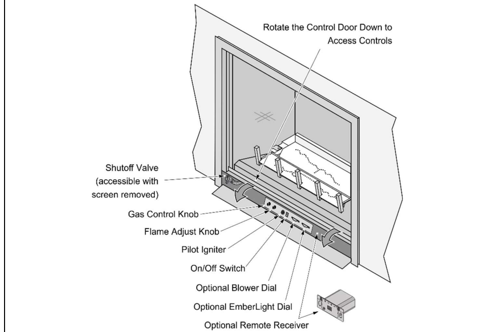
MV Version
