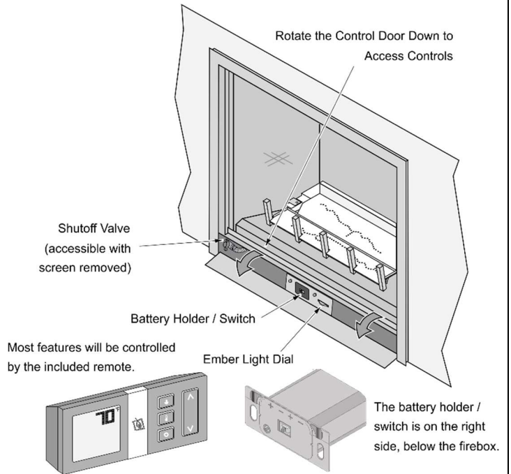
GSR2 Version
