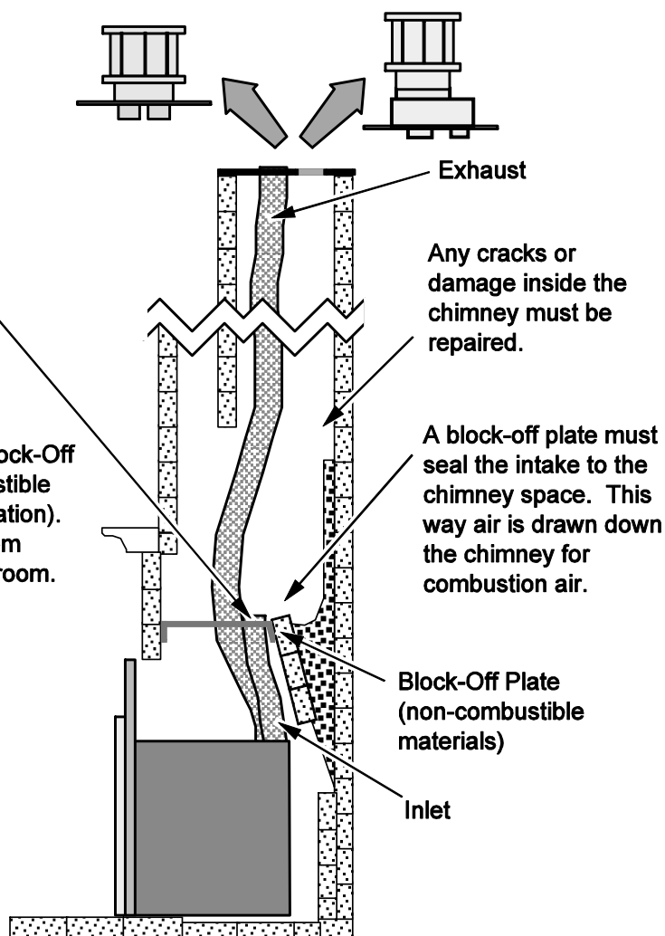
Masonry Fireplace
