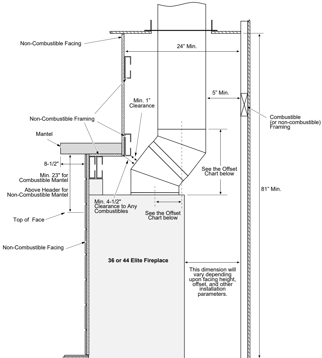
OFFSET CHART
